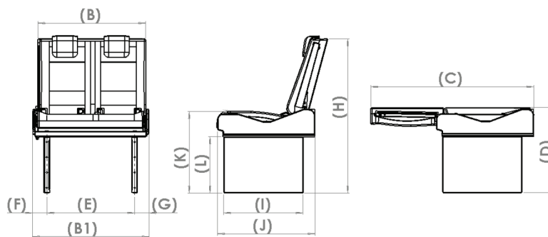
ILGAZ Models - Seat & Bench Combinations Dimensions (without rear bed)
