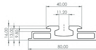
230720251554STRAY 13mm Slim Rail Profile (NEW)
