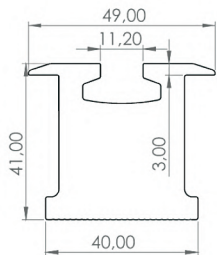
170220231522STKT 38mm Rail Profile 3450 gr
