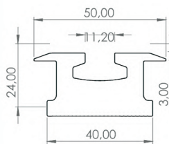
140220231457STKT 21mm Rail Profile 1950 gr
