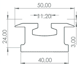
140220231457STKT 21mm Rail Profile 1950 gr
