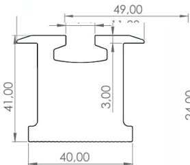
170220231522STKT 38mm Rail Profile 3450 gr
